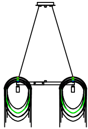
A Fixture Body x1
